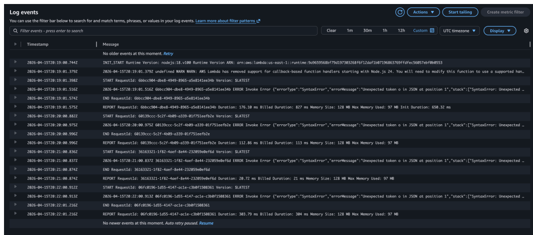
Figure 1.4: Post-fix CloudWatch logs confirming injected payload no longer executes
